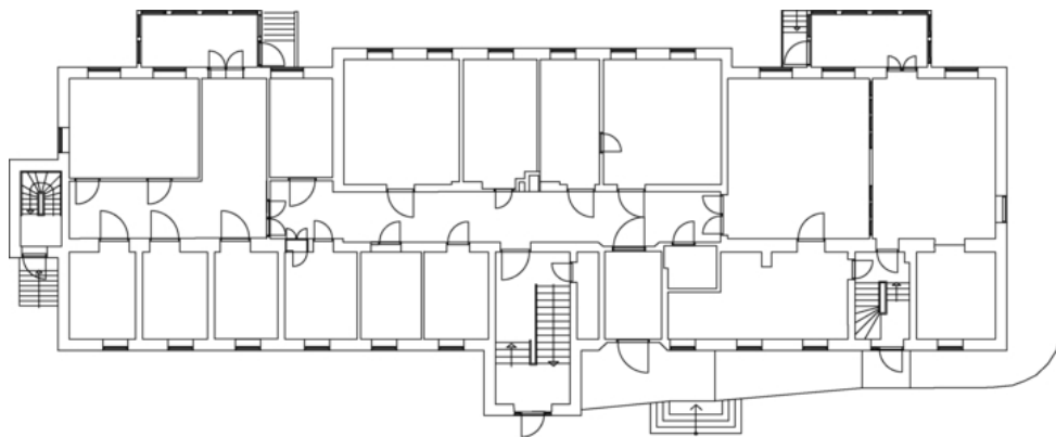
2106, Post 6, 1.etg.
