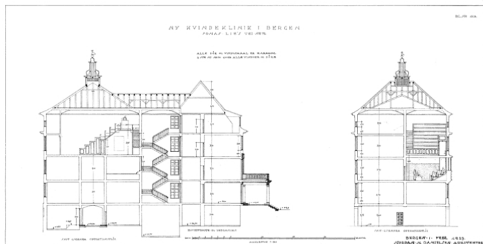
Original snittegning.
