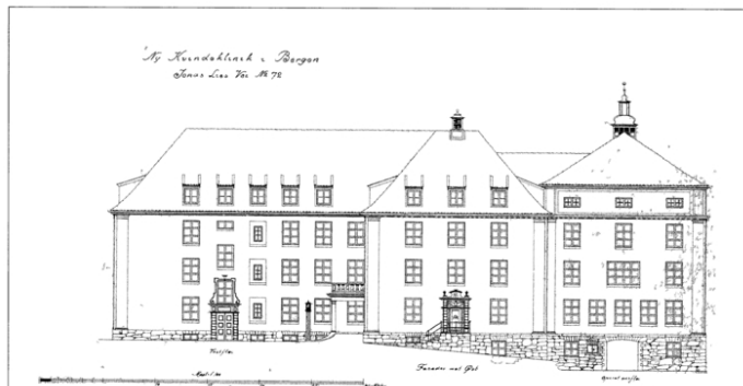
Original fasadetegning.
